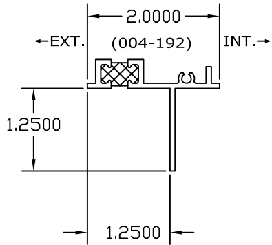
1800 SERIES NAIL FIN 2" FRAME ADAPTER
