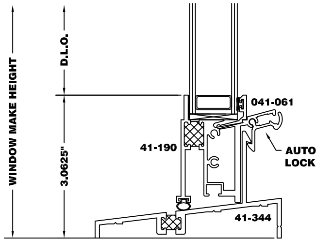
Frame Options: 1/2" Ext. Leg Sill (QX)
