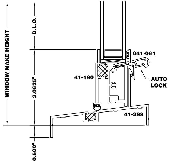
Frame Options: 1/2" Ext. Leg Sill (XX)
