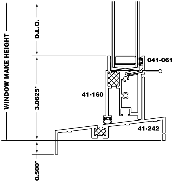
Frame Options: 1/2" Ext. Leg Sill (XR)
