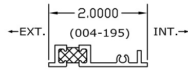
1800 SERIES (FALSE) NAIL FIN 2" FRAME ADAPTER
