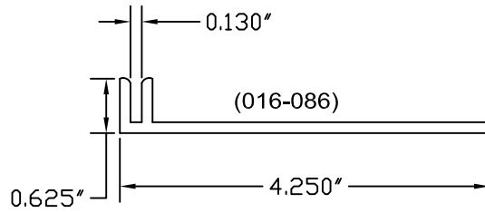
F - STRAP ANCHOR
