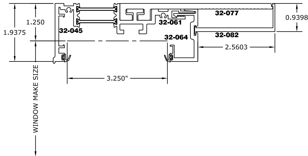
(G3/4RC) 3 1/4"-G300/G400 TWO PIECE RECEPTOR SYSTEM W/STRAP ANCHOR W TRIM COVER
