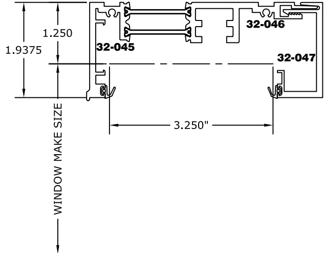
(G3/4RA-125) 3 1/4"-G300/G400 TWO PIECE RECEPTOR SYSTEM
