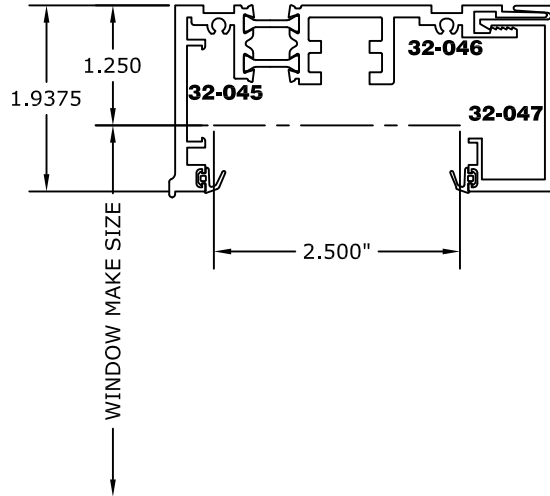
(G1RA-125) 2 1/2"-G100 TWO PIECE RECEPTOR SYSTEM
