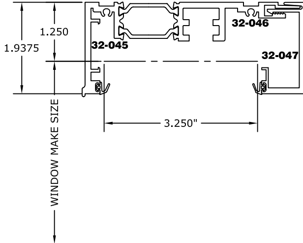
(G2RA-125) 3 1/4"-G200 TWO PIECE RECEPTOR SYSTEM
