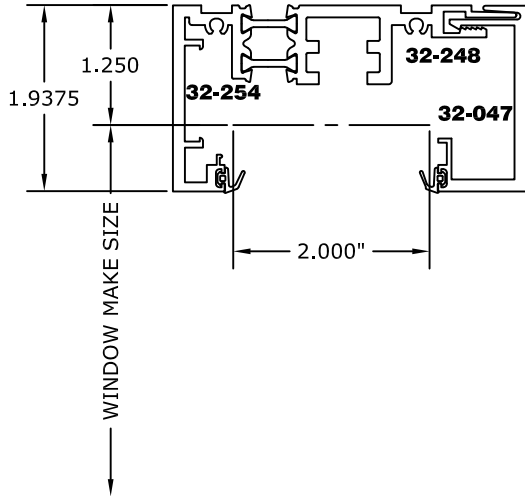
(G0RA-125) 2"-G000 TWO PIECE RECEPTOR SYSTEM
