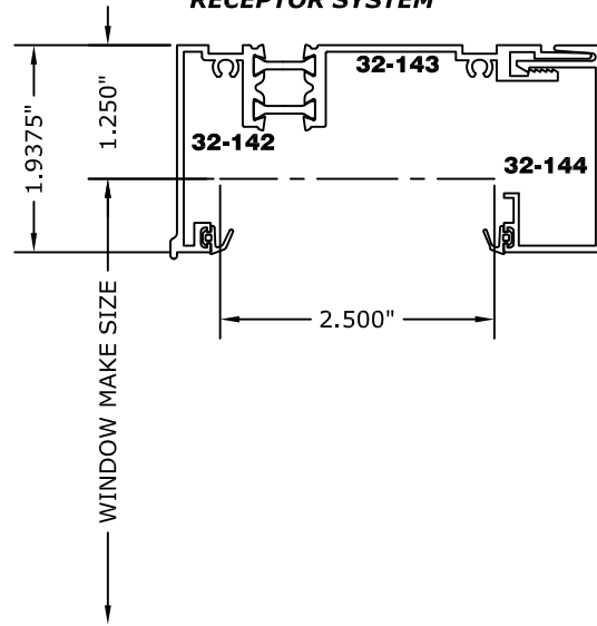
(G1RA) 2 1/2"-G100 TWO PIECE RECEPTOR SYSTEM
