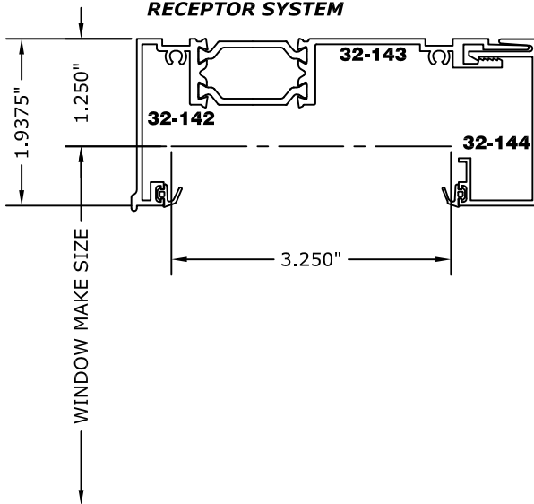
(G2RA) 3 1/4"-G200 TWO PIECE RECEPTOR SYSTEM
