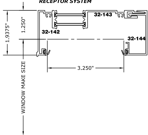
(G3/4RA) 3 1/4"-G300/G400 TWO PIECE RECEPTOR SYSTEM
