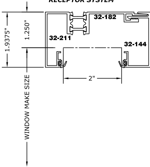
(G0RB) 2"-G000 TWO PIECE RECEPTOR SYSTEM
