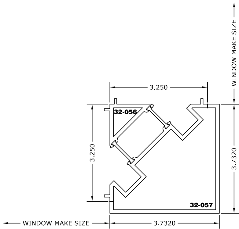
(G3/4MD) 3 1/4"-G300/G400 90 Deg. Corner Mullion
