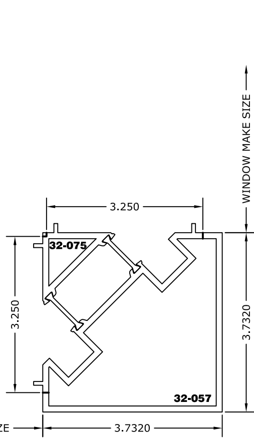
(G2MD) 3 1/4"-G200 90 Deg. Corner Mullion
