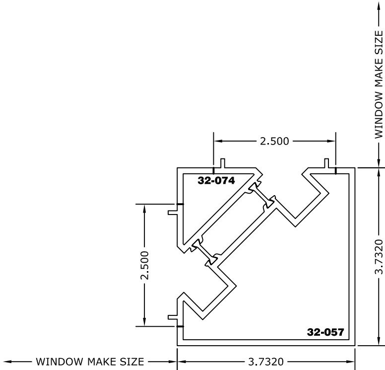
(G1MD) 2 1/2"- G100 90 Deg. Corner Mullion
