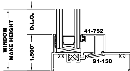
Frame Options: Sill (QR) **Used for Model 9635 Only**
