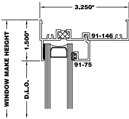
Frame Options: Head/Jambs/Sill
