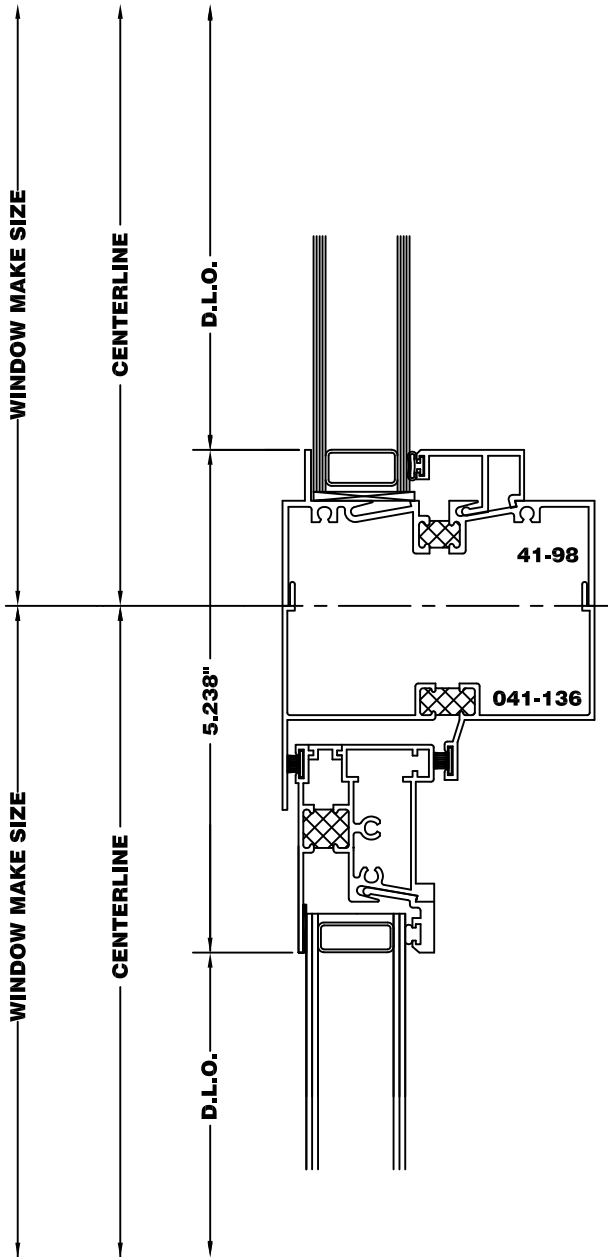
Model 4160 Fixed Over 4320/4330 Single Hung 3 1/4" Frame Depth
