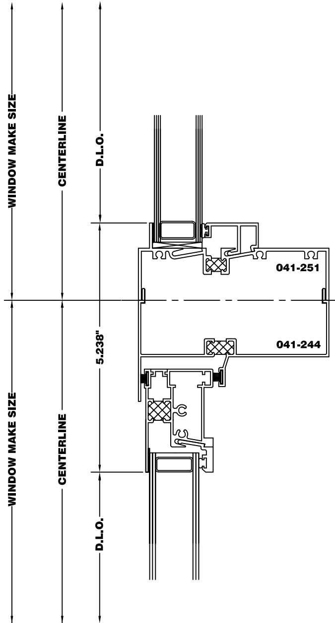
Model 4170 Fixed Over 4340/4350 Single Hung 4" Frame Depth
