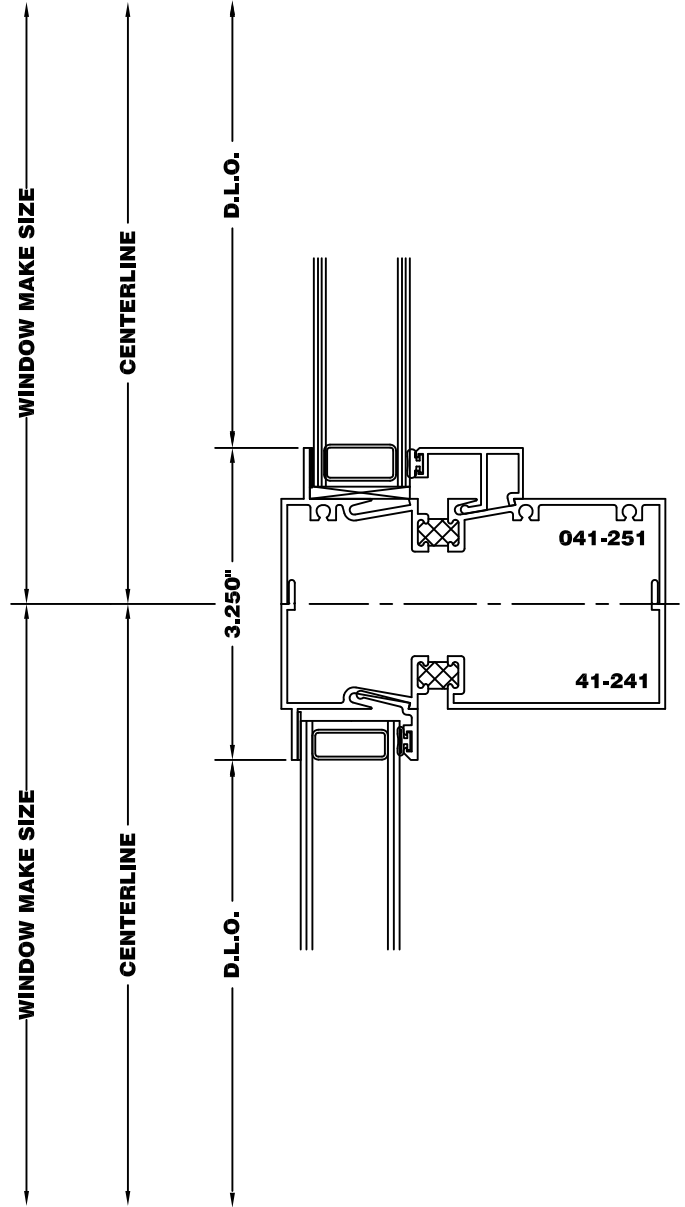
Model 4170 Fixed Over 4140/4150 Single Hung 4" Frame Depth
