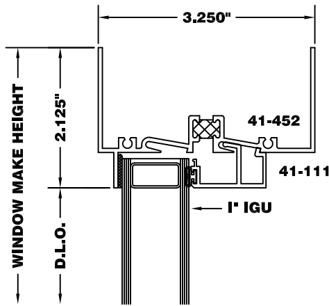
Frame Options: Head/Jambs/Sill
