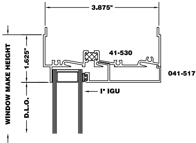
Frame Options: Head Typ. Used w/ Offset Glazing
