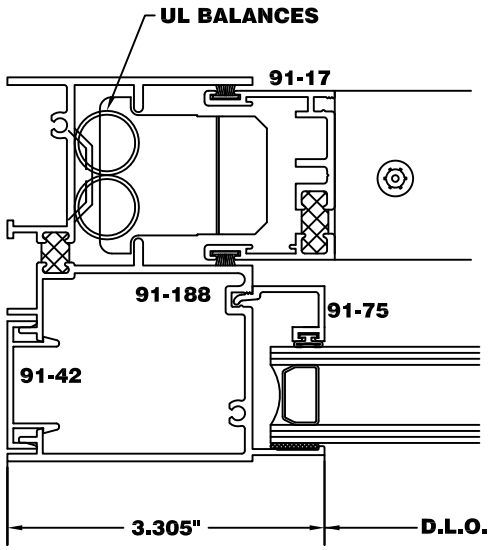
Frame Option: Jambs w/o Screen Leg
