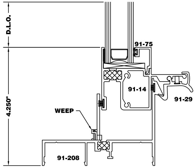
Model 915W Sill Option: QR Sill
