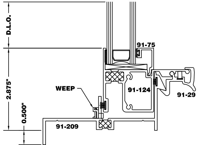
Model 915W Sill Option: XR Sill
