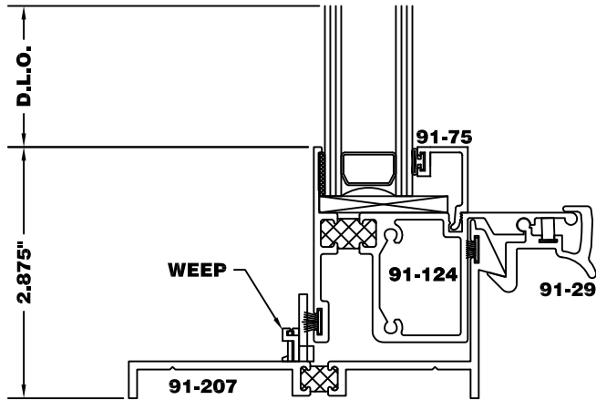
Model 915W Sill Option: QR Sill
