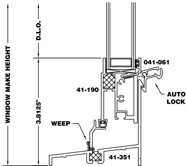
Frame Options: 1/2" Ext. Leg Sill (QX)
