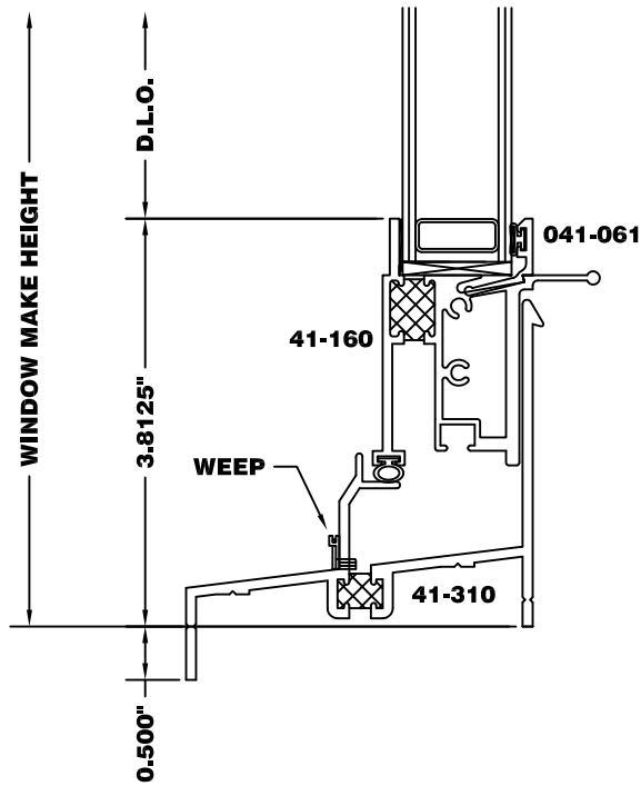
Frame Options: 1/2" Ext. Leg Sill (XR)
