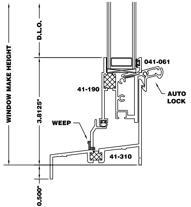
Frame Options: 1/2" Ext. Leg Sill (XX)
