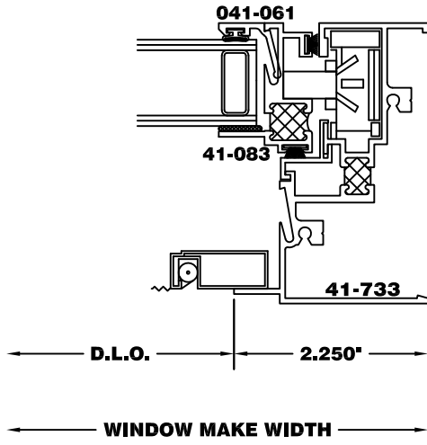
Frame Options: Jamb w/o Nail Fin (Can be used at Head-Model 4125 Only)
