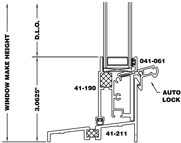
Frame Options: 1/2" Ext. Leg Sill (QX)
