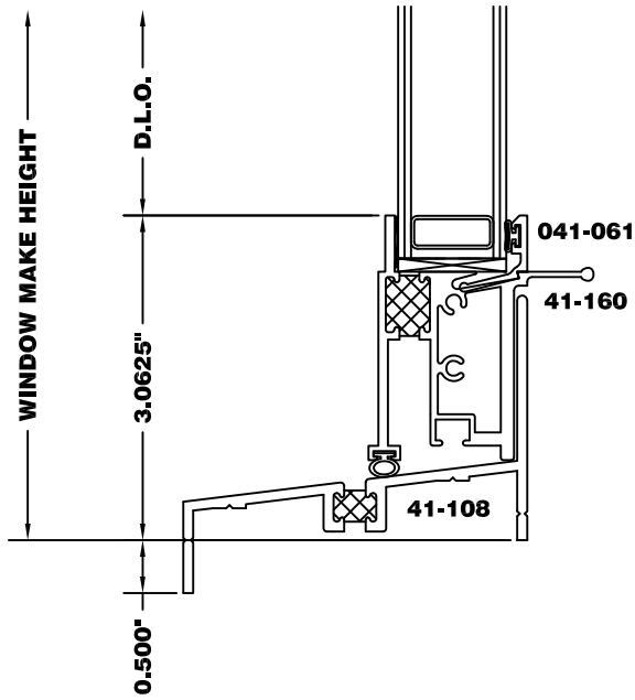
Frame Options: 1/2" Ext. Leg Sill (XR)
