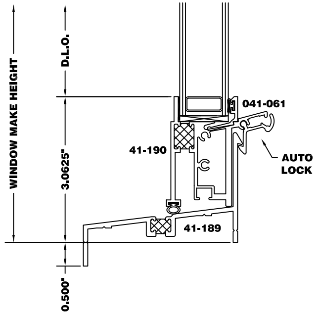
Frame Options: 1/2" Ext. Leg Sill (XX)
