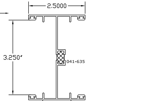
(041-635) 3 1/4" H- Mullion
