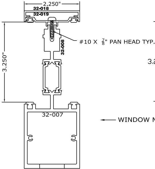
(4139) 3 1/4" -3 Piece Mullion
