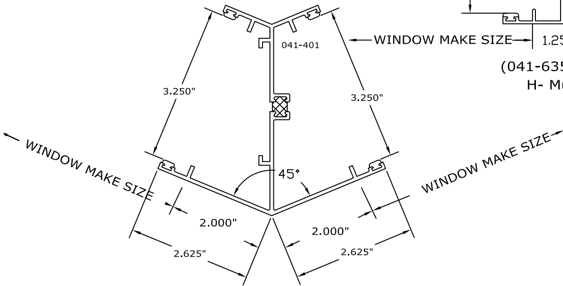
(41-401) 45 Deg. Mullion
