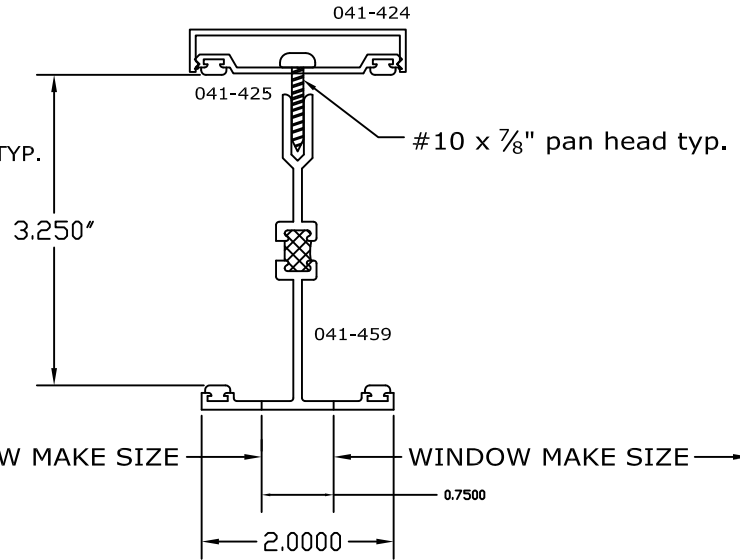
(4139) 3 1/4" -3 Piece Mullion
