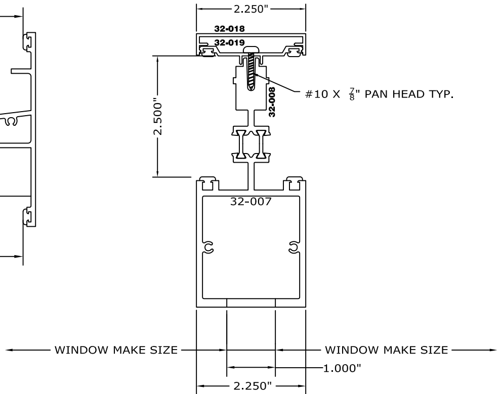
(0418) 2 1/2" TUBE- MULLION
